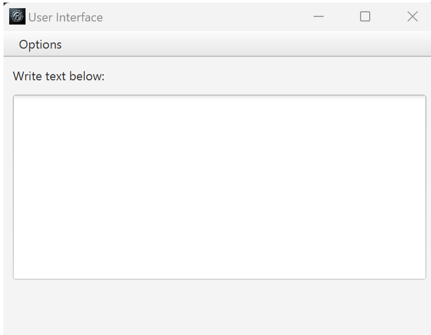
Figure 1 Welcome Window
